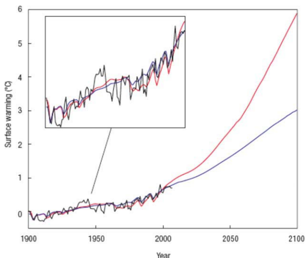
Figure 7. Simulation of observed warming over the 20th Century with a low climate sensitivity and high net forcing (2°C, 2.5 W m -2 ; blue line) and a high climate sensitivity and low net forcing (6°C, 1.4 W m -2 ; red line).
