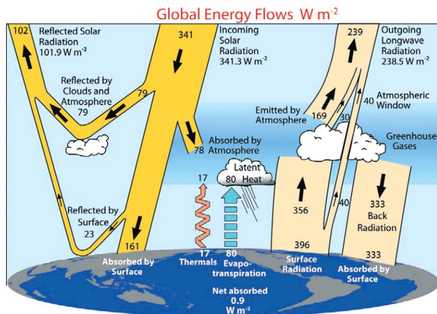
Figure 1. Earth's energy balance. 3 Incoming and outgoing energy fluxes from Earth on an annual-average basis.
